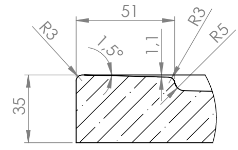
DETAIL E SCALE 1 : 2
