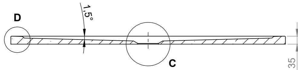
SECTION B-B
