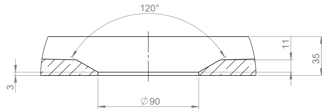
DETAIL E SCALE 1 : 2
