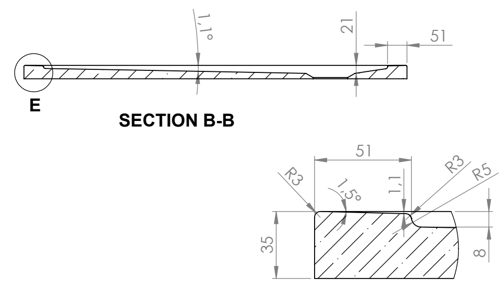
DETAIL E SCALE 1 : 2
