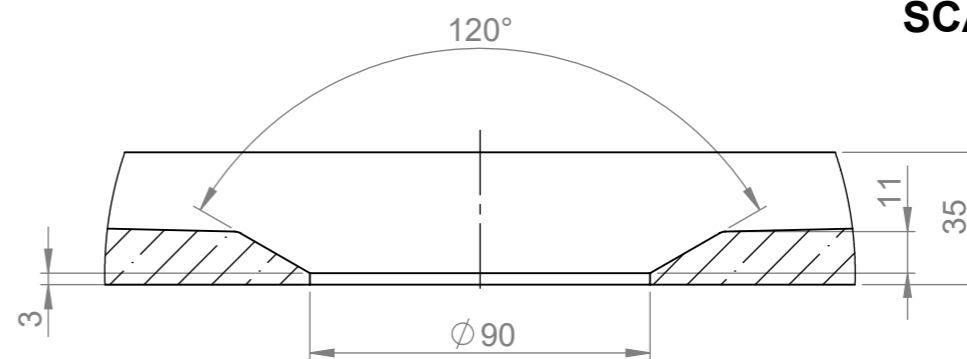
DETAIL C SCALE 1 : 2
