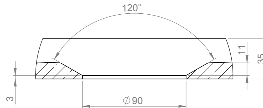
DETAIL C SCALE 1 : 2
